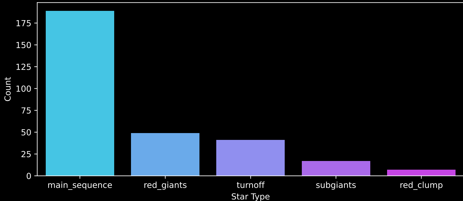
APOGEE DR17 Field: [220+55_btx] Count plot of Star Type
