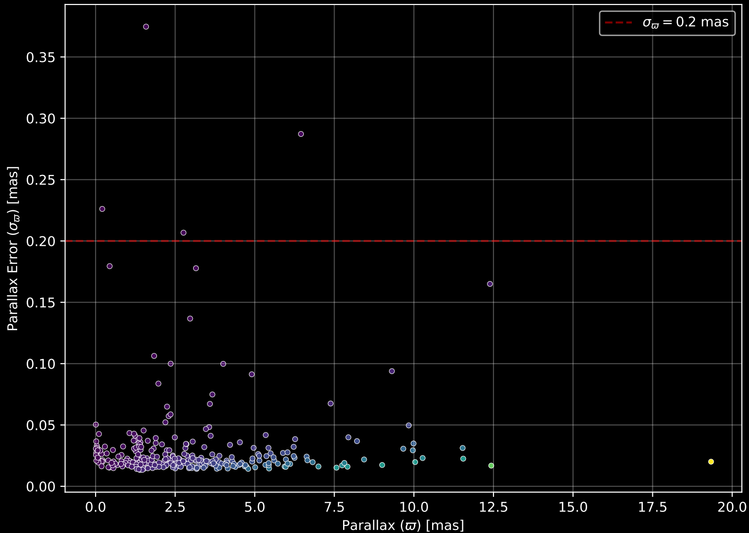
APOGEE DR17 Field: [220+55_btx] Parallax Quality (n= 303)
