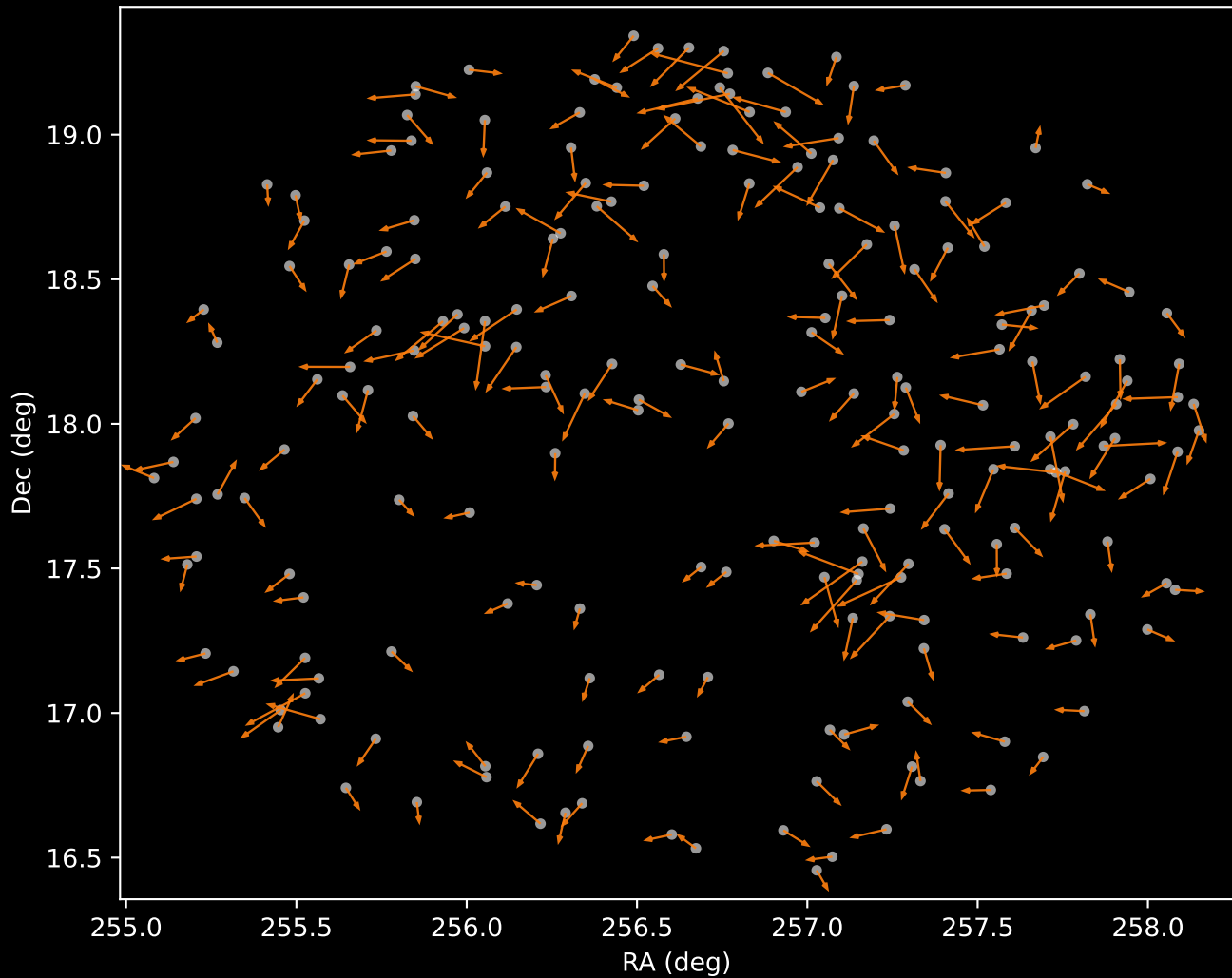
APOGEE DR17 Cluster 2 Proper Motion Vectors (n=214)
