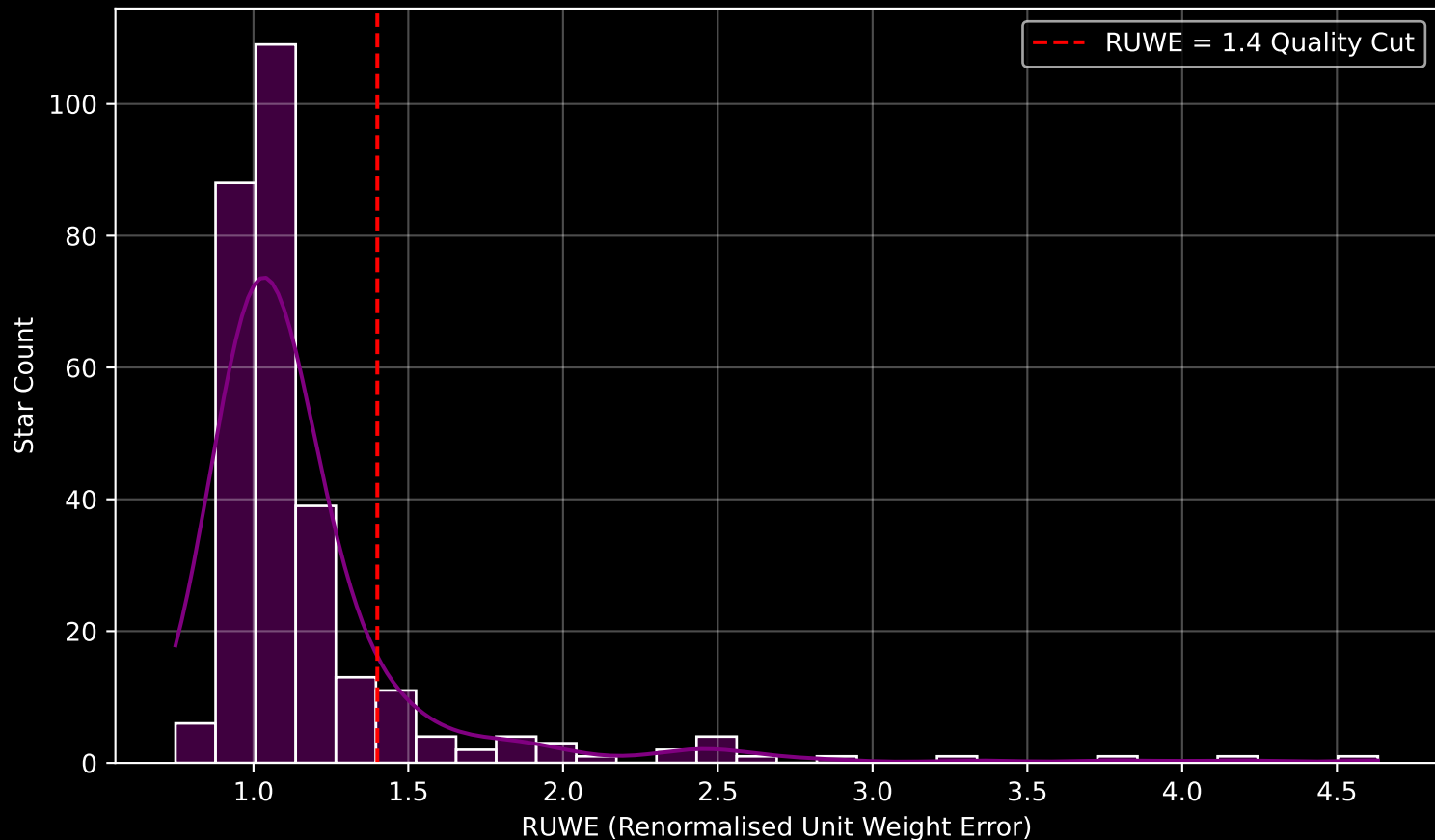
GAPOGEE DR17 Field [220+55_btx] RUWE Distribution (n= 292)
