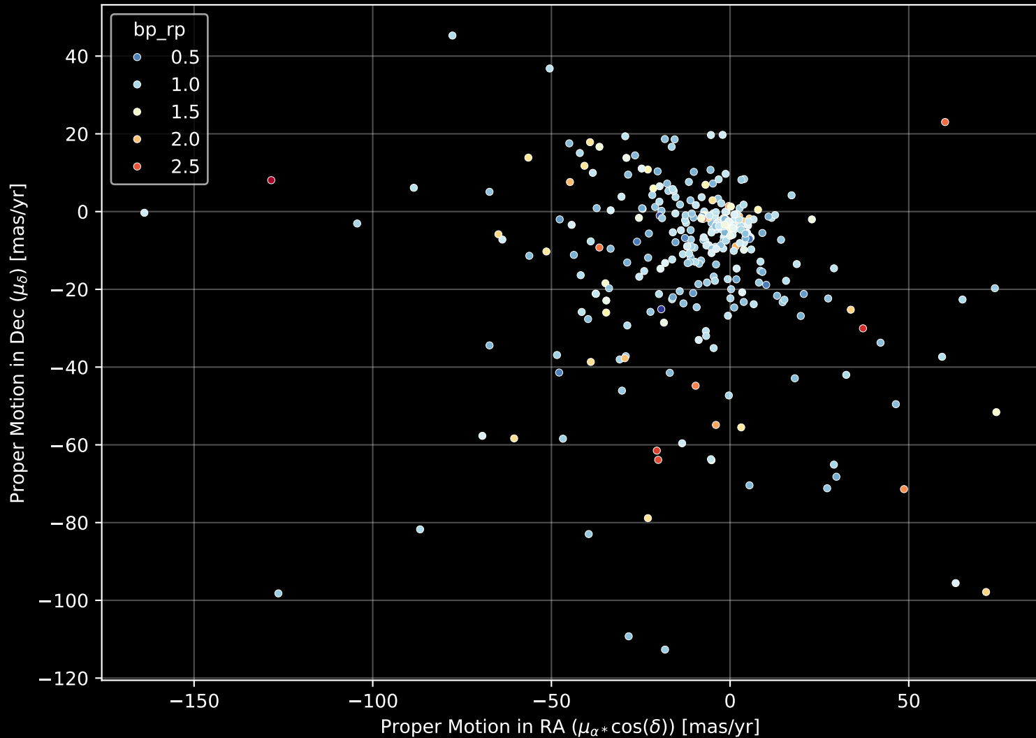
APOGEE DR17 Field: [220+55_btx] Proper Motion Diagram (n= 303)
