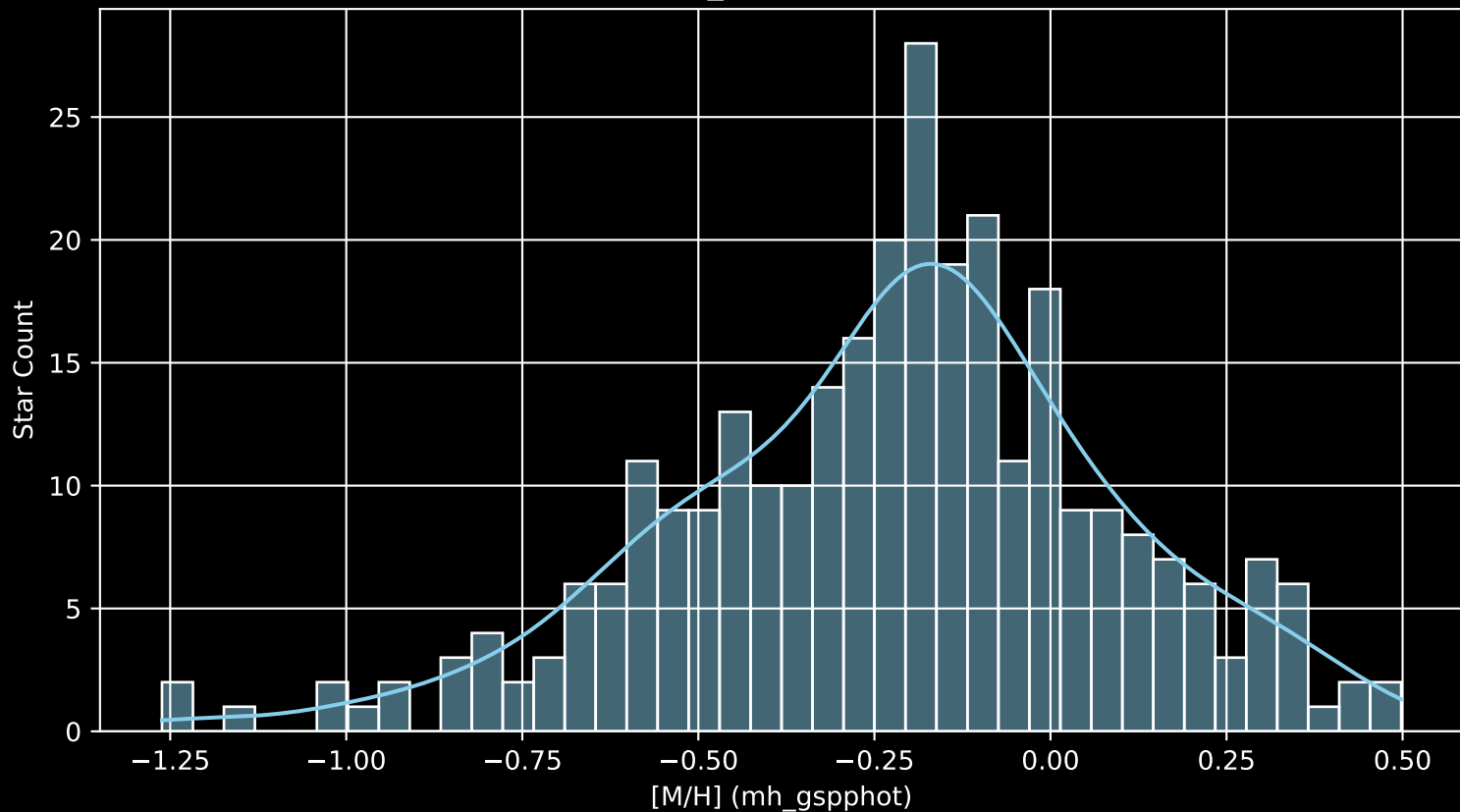
APOGEE DR17 Field: [220+55_btx [M/H] (mh_gspphot) (n= 301)
