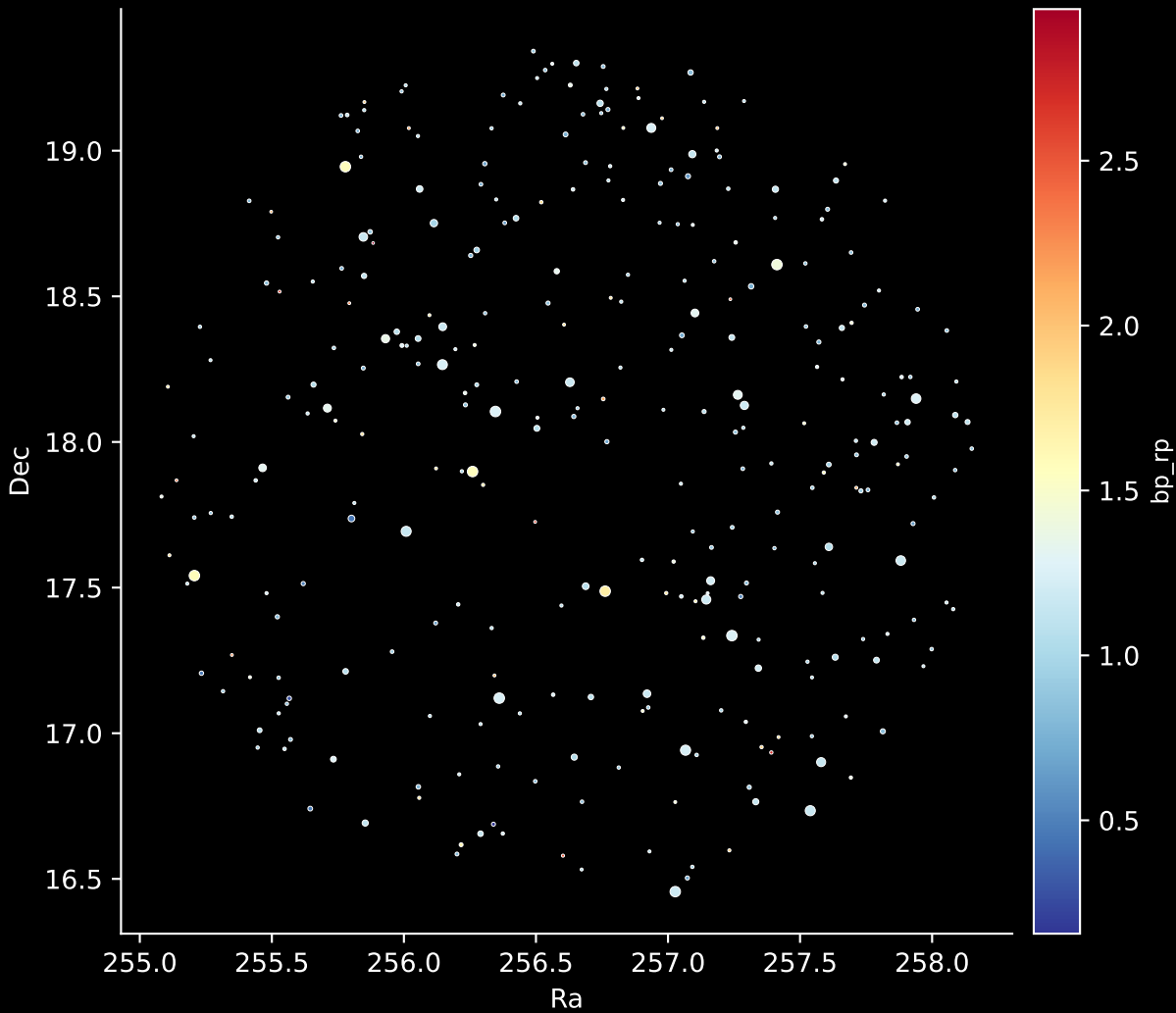
APOGEE DR17 Field: [220+55_btx] Stars: 303
